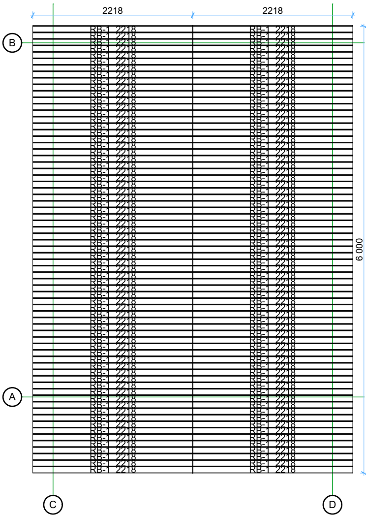
Roof boards
